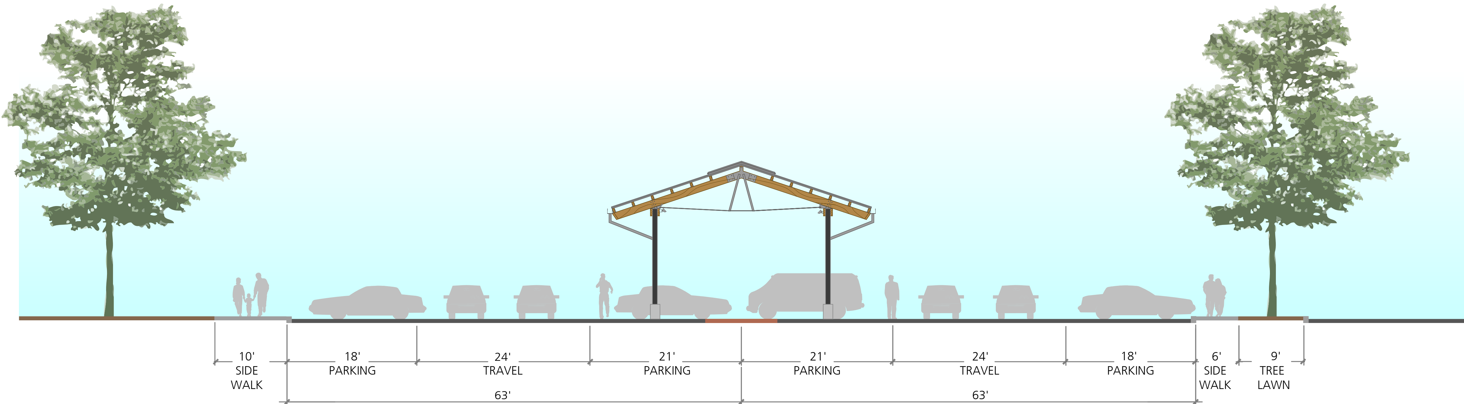
Market Shed Cross Section - Non-Market Days
