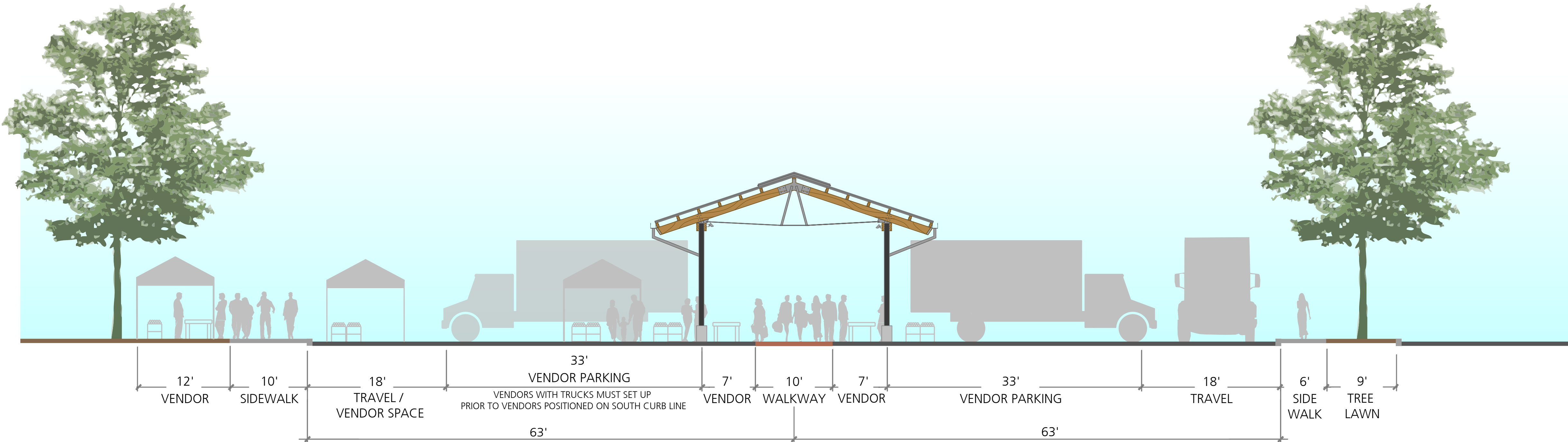
Market Shed Cross Section - Market Days
