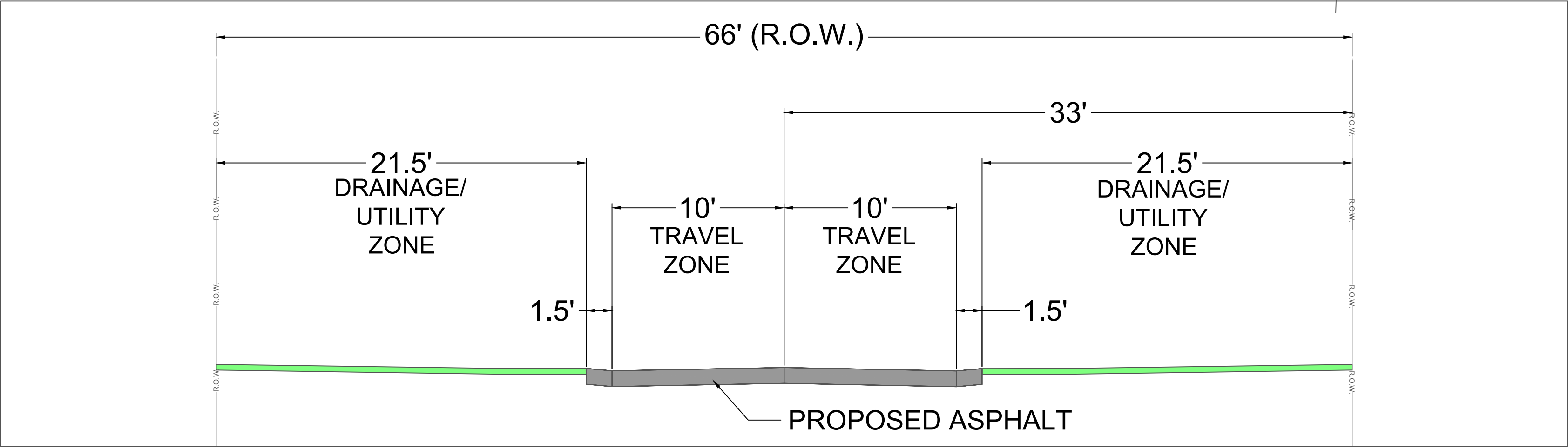
PROPOSED SECTION A-A
